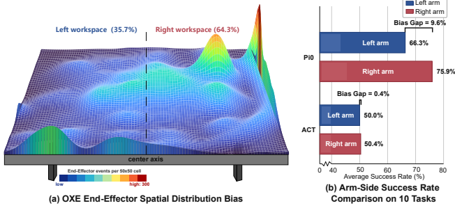
Fig. 2. Arm-side spatial preference analysis in robot data and policies. (a) End-effector workspace distribution estimated from Open X-Embodiment trajectories. (b) Left- and right-arm performance comparison of pretrained \pi_0 and non-pretrained ACT across 10 RoboTwin 2.0 tasks, examining whether data-level spatial imbalance is reflected in downstream policy performance.
