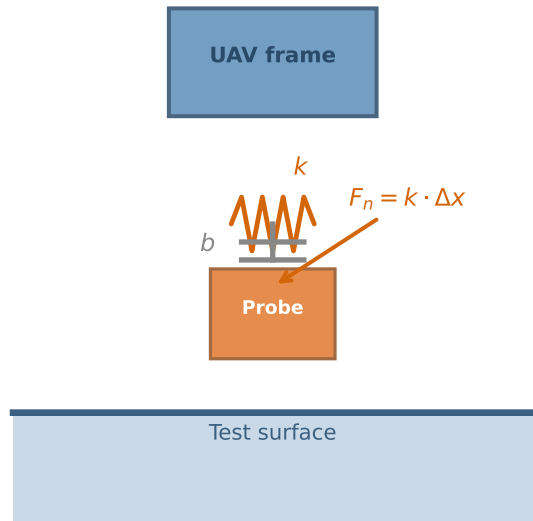
(a) Passive compliant mechanism
