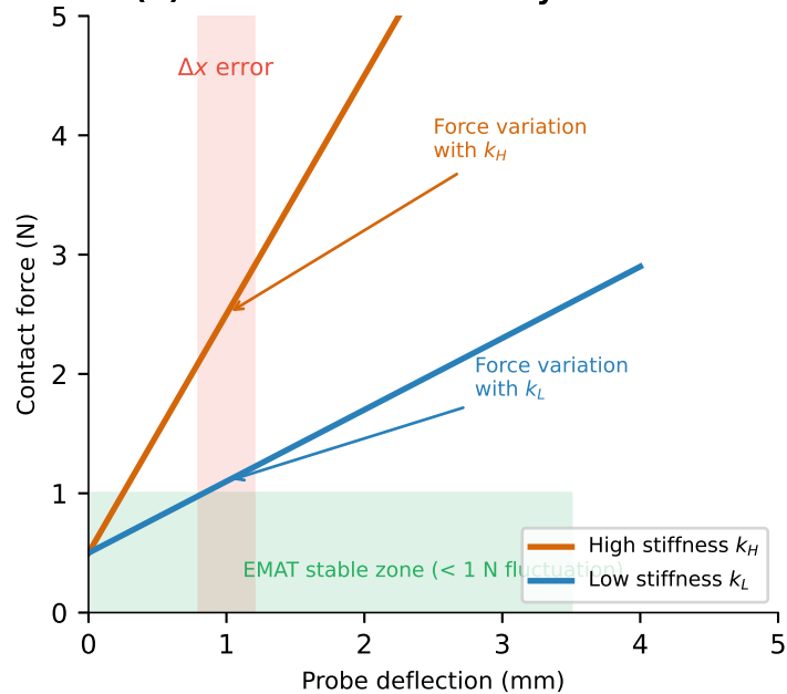
(b) Force uncontrolled by deflection
