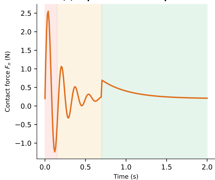
(c) Impact transient response
