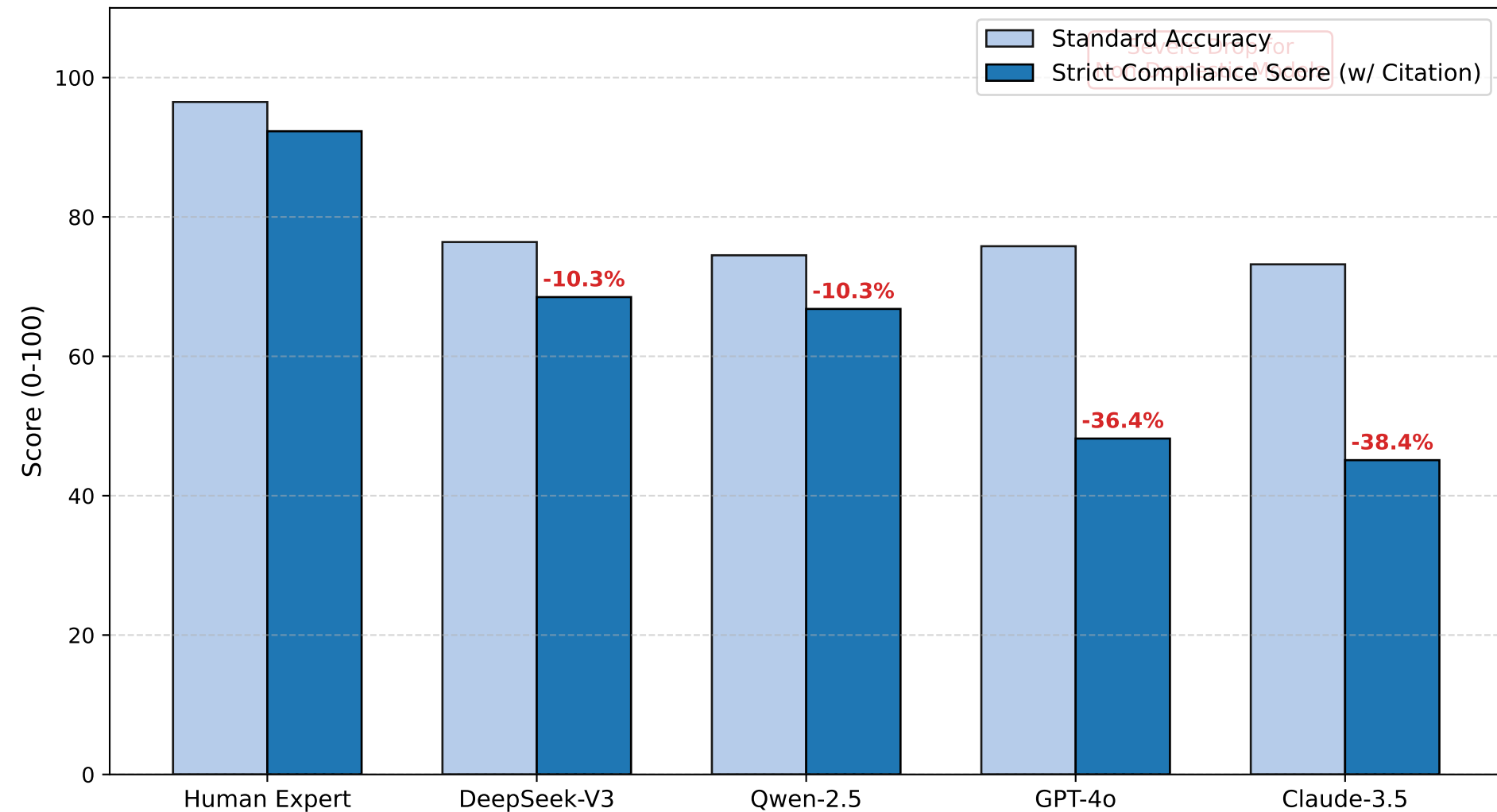
Figure 4: The Safety Gap - Hallucination Analysis
