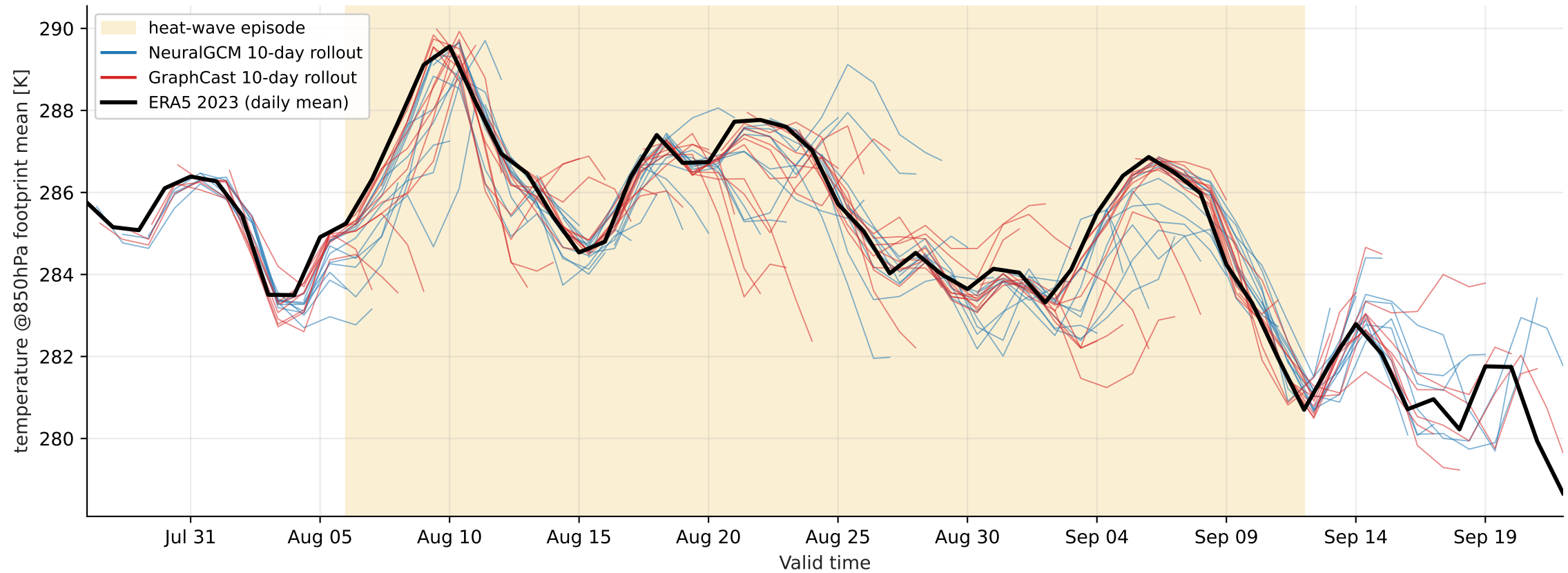
Europe heat-wave 2023-08-06..2023-09-12 — footprint-mean temperature @ 850 hPa (cordex, > p99)
