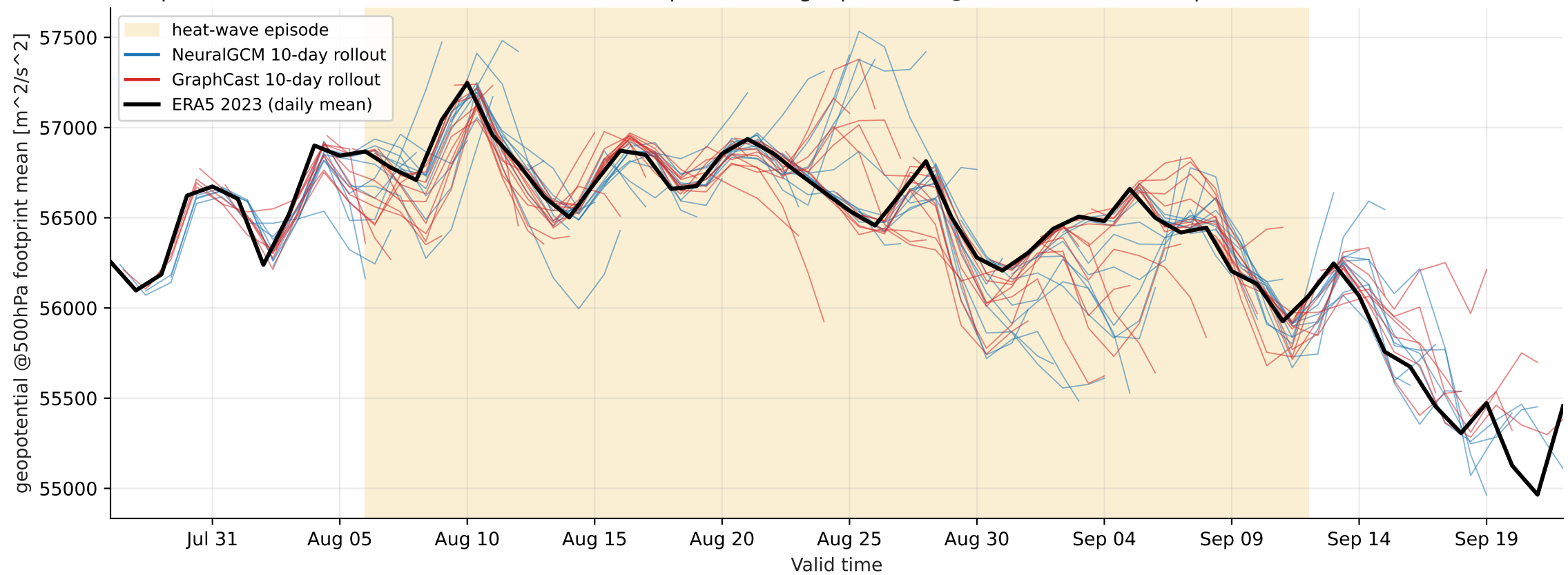
Europe heat-wave 2023-08-06..2023-09-12 — footprint-mean geopotential @ 500 hPa (cordex, > p99)
