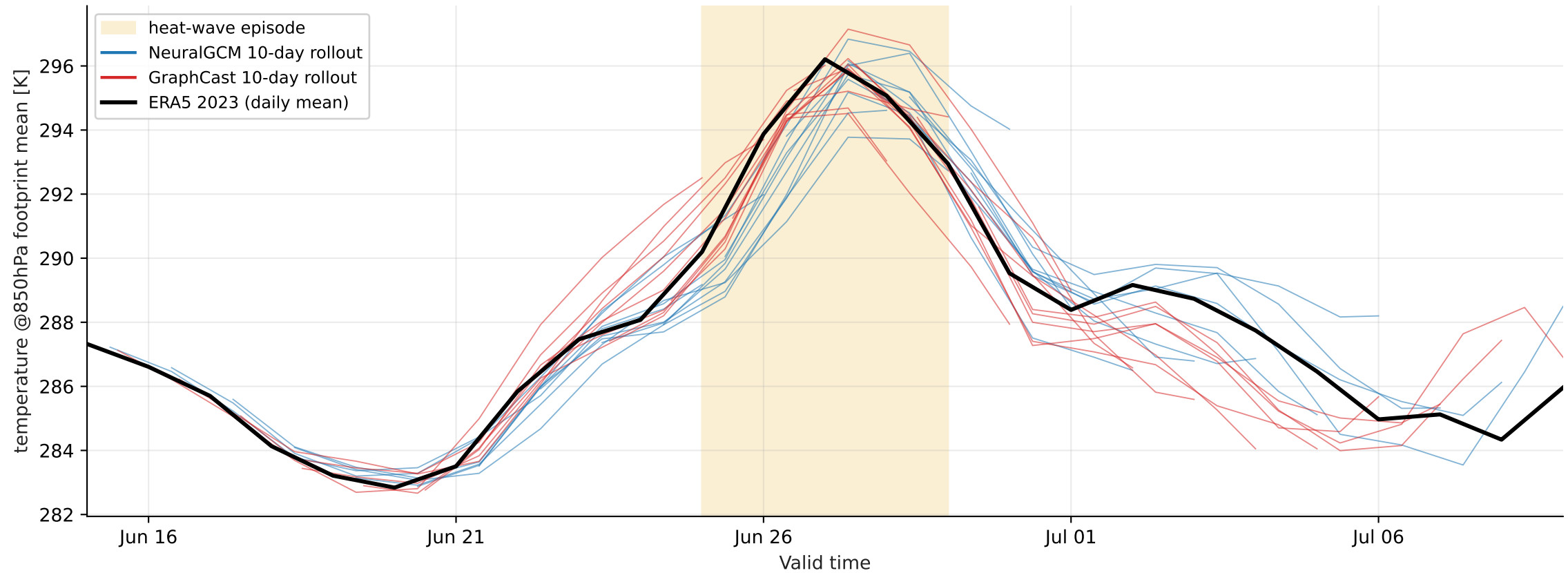
Europe heat-wave 2023-06-25..2023-06-29 — footprint-mean temperature @ 850 hPa (mixture, > p99)
