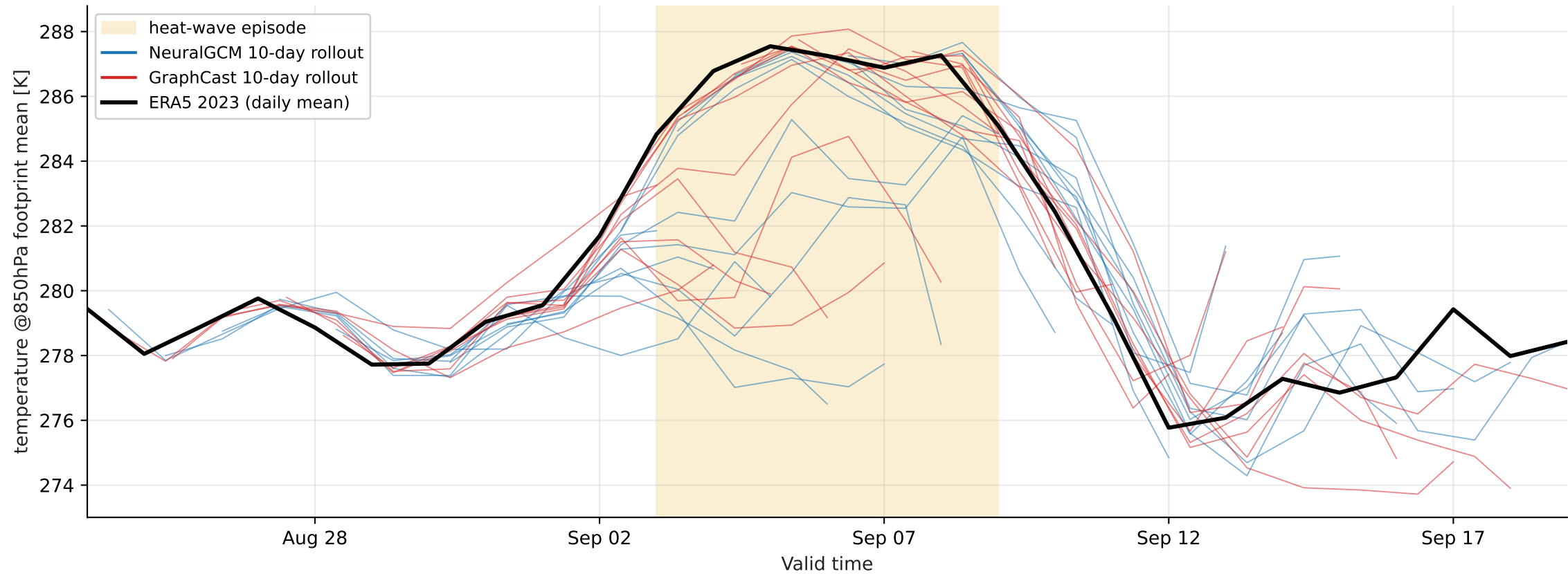
Europe heat-wave 2023-09-03..2023-09-09 — footprint-mean temperature @ 850 hPa (mixture, > p99)
