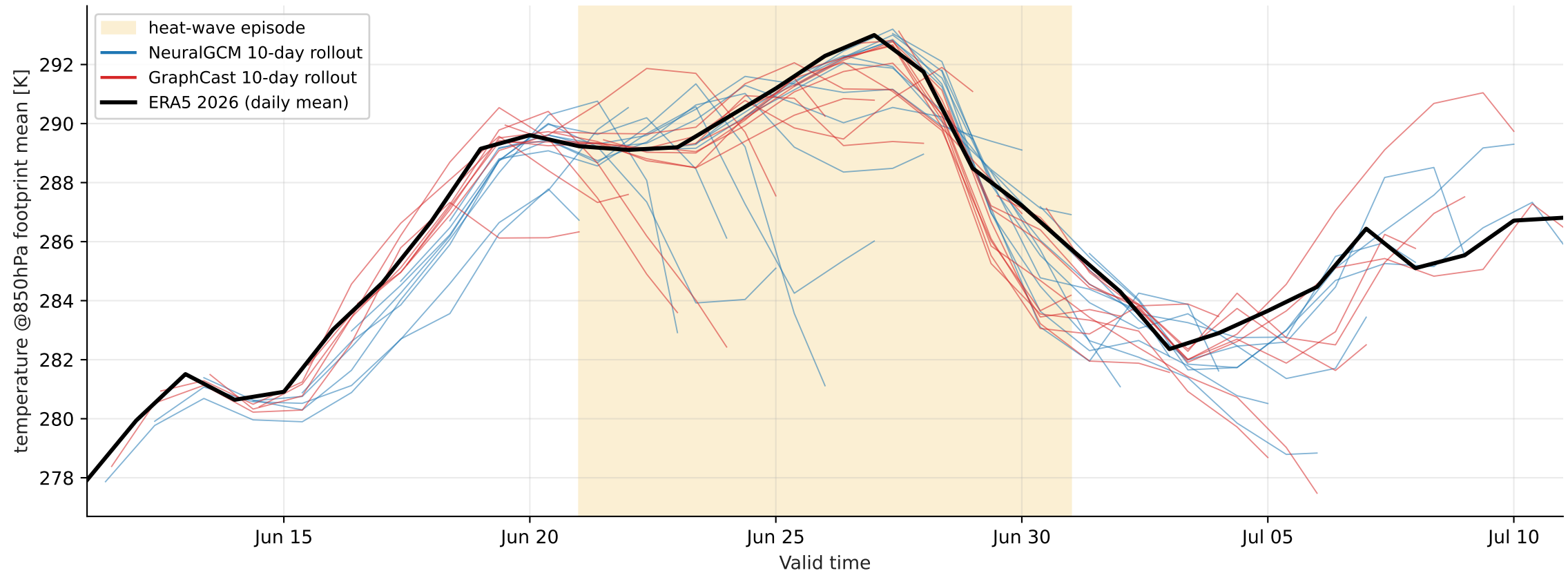
Europe heat-wave 2026-06-21..2026-07-01 — footprint-mean temperature @ 850 hPa (mixture, > p99)
