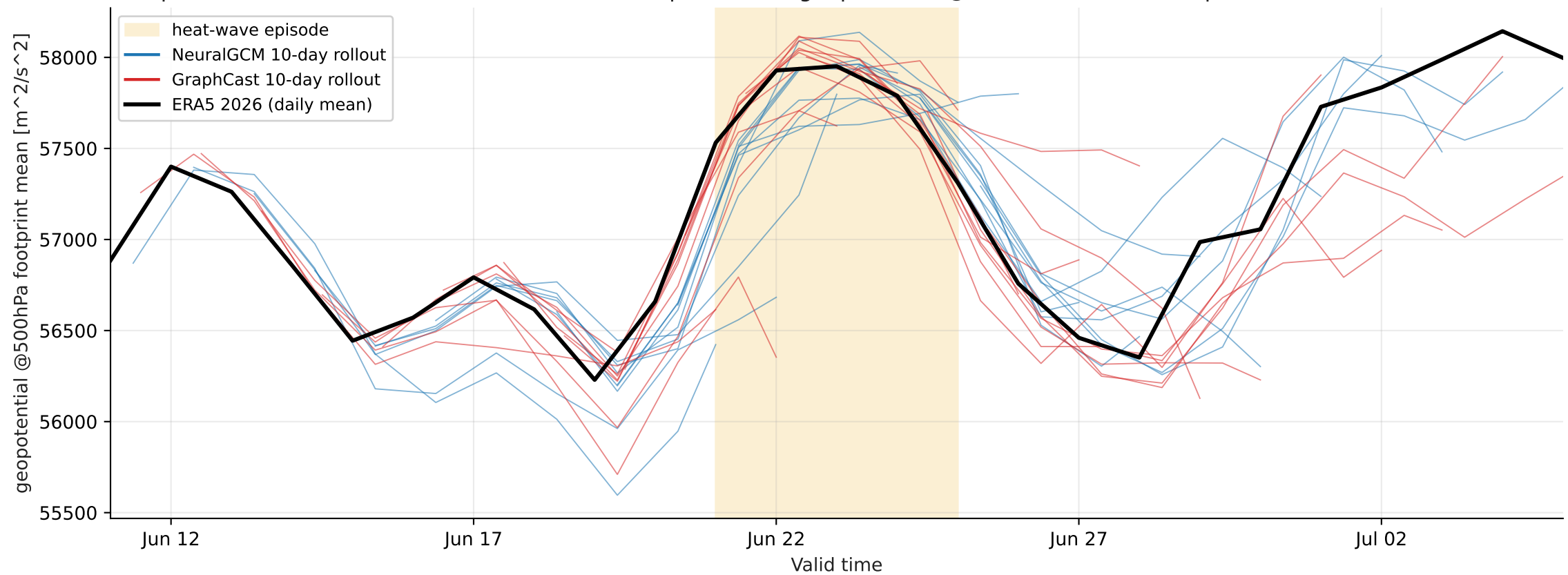
Europe heat-wave 2026-06-21..2026-06-25 — footprint-mean geopotential @ 500 hPa (mixture, > p99)
