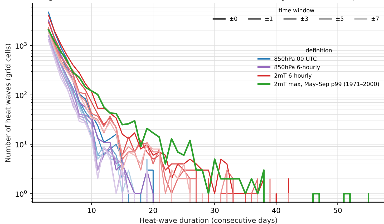
Length of heat wave classification in the world in 2026 by definitions (> p99)
