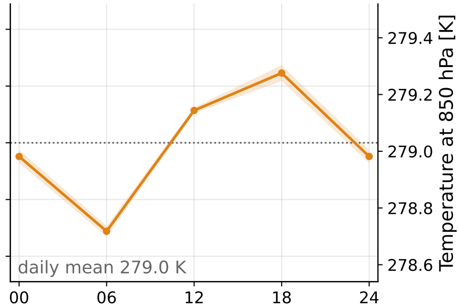
NextGEMS-2049
