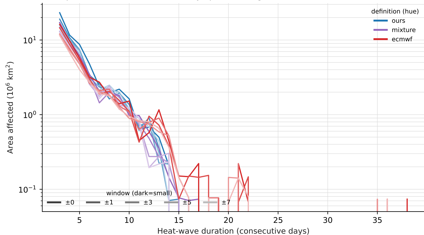
Europe — 2026 heat waves by definition & window — area 95th-pctile, 1991-2020 ref, \geq 3 -day spells, 2.8^\circ grid
