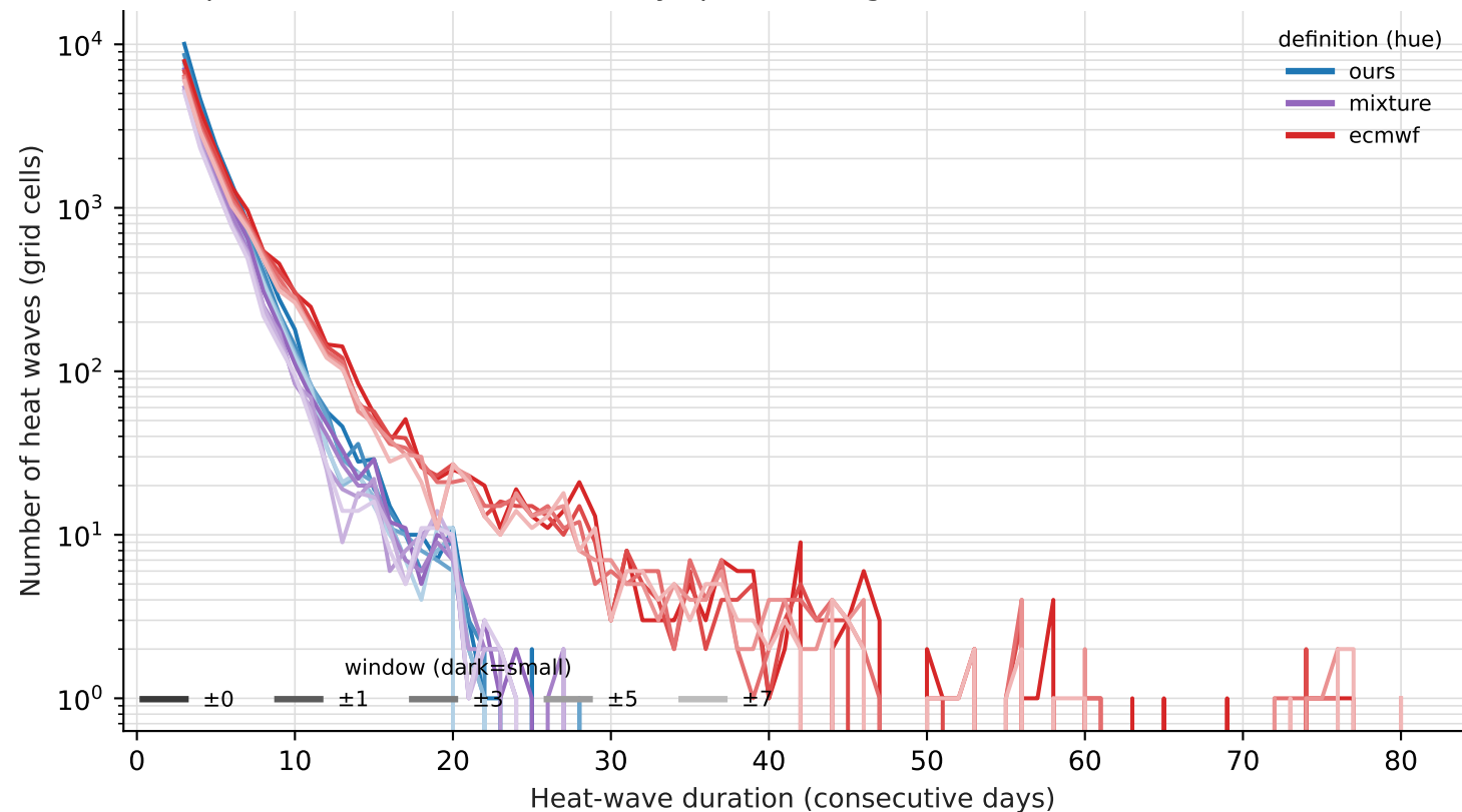
2026 heat waves by definition & window — count 95th-pctile, 1991-2020 ref, \geq 3 -day spells, 2.8^\circ grid
