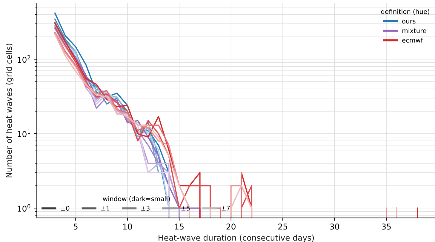
Europe — 2026 heat waves by definition & window — count 95th-pctile, 1991-2020 ref, \geq 3 -day spells, 2.8^\circ grid
