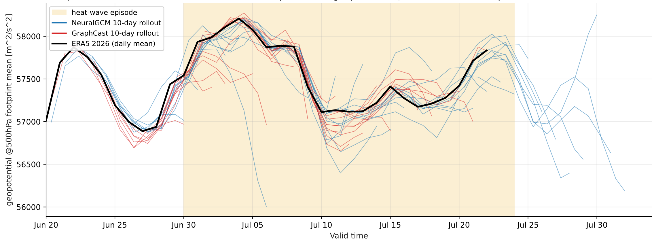
Europe heat-wave 2026-06-30..2026-07-24 — footprint-mean geopotential @ 500 hPa (cordex, > p99)
