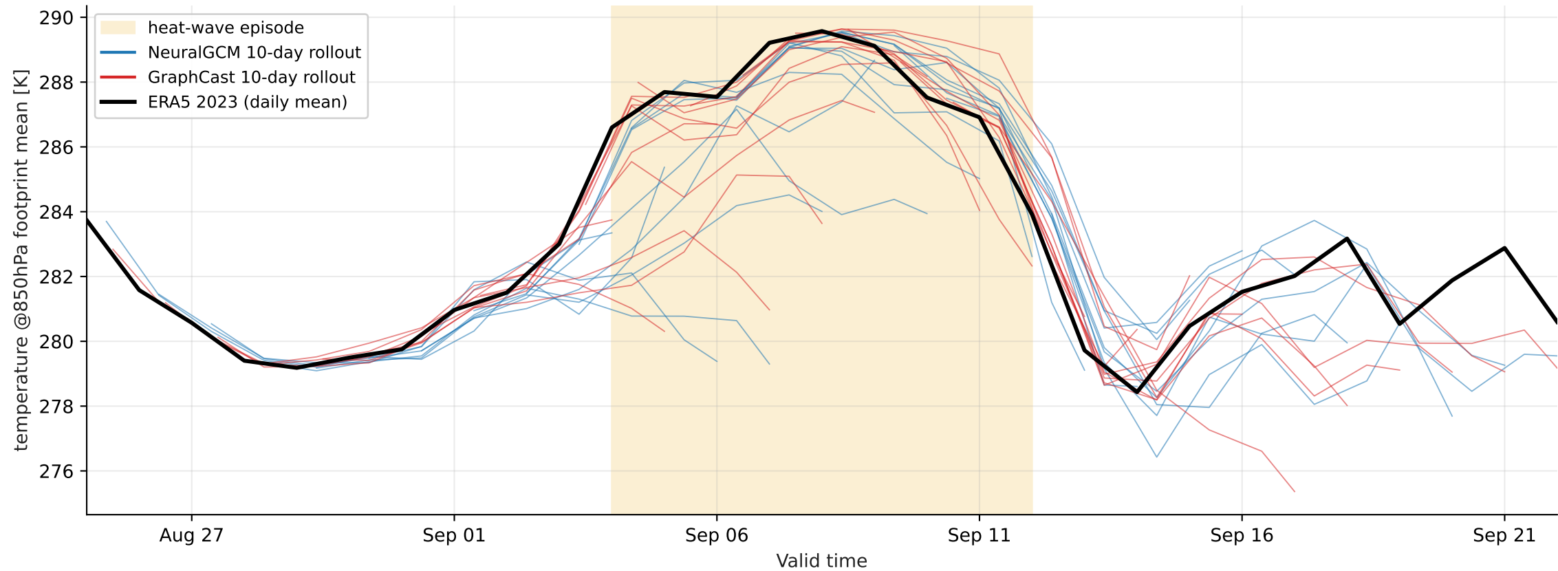
Europe heat-wave 2023-09-04..2023-09-12 — footprint-mean temperature @ 850 hPa (mixture, > p99)
