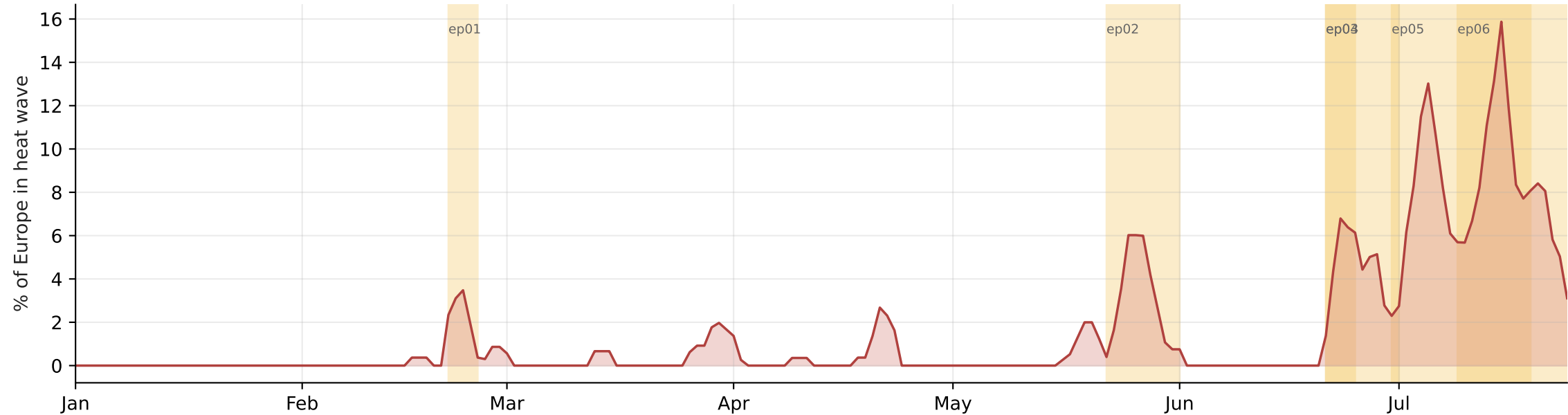
Europe heat-wave coverage in 2026 (mixture > p99, 6 episodes)
