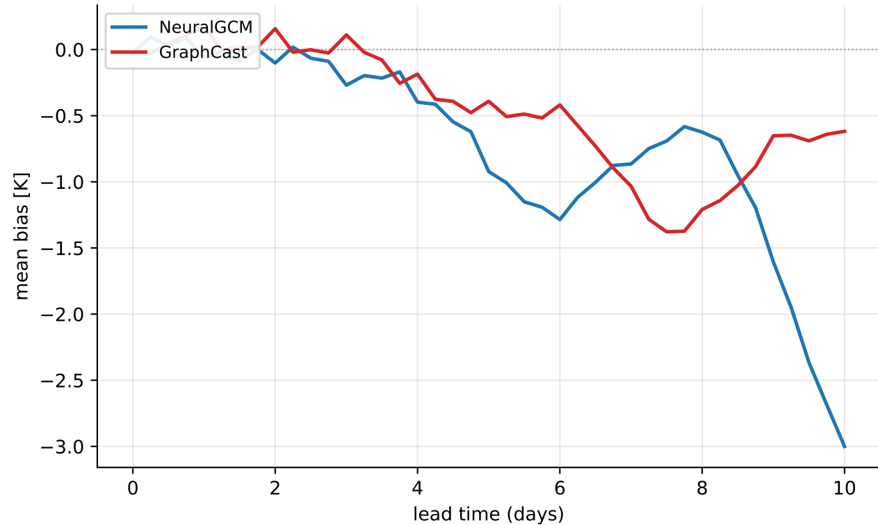
Europe heat-wave 2026-06-21..2026-06-25 — footprint temperature@850 hPa (mean of 15 rollouts)
