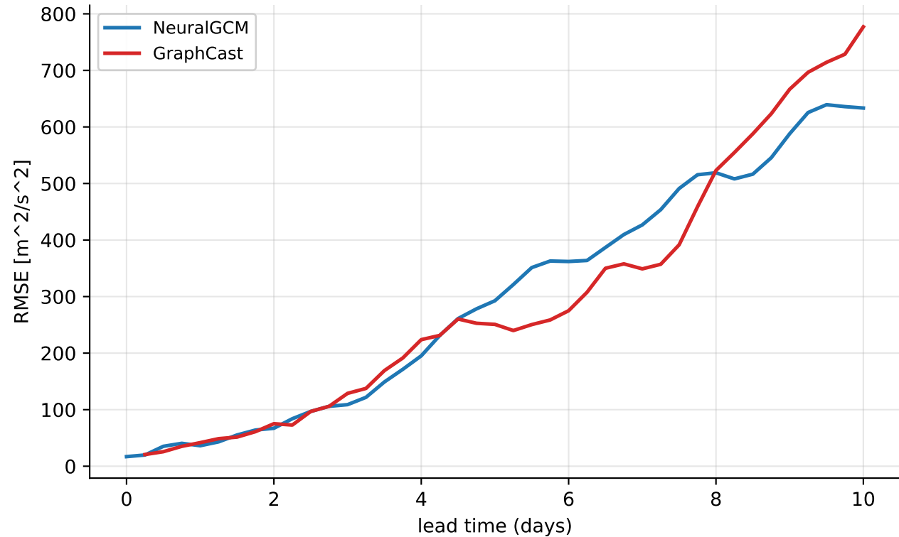
Europe heat-wave 2026-06-21..2026-06-25 — footprint geopotential@500 hPa (mean of 15 rollouts)
