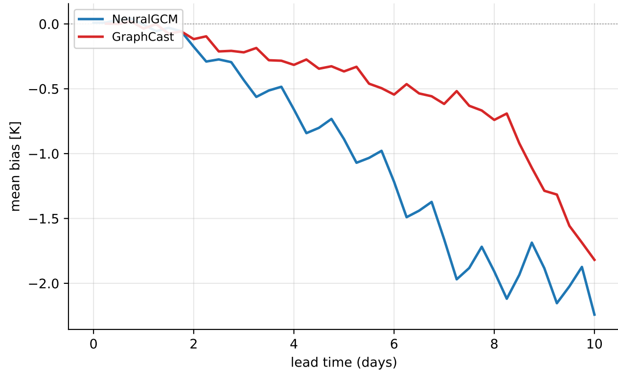
Europe heat-wave 2026-07-09..2026-07-24 — footprint temperature@850 hPa (mean of 14 rollouts)
