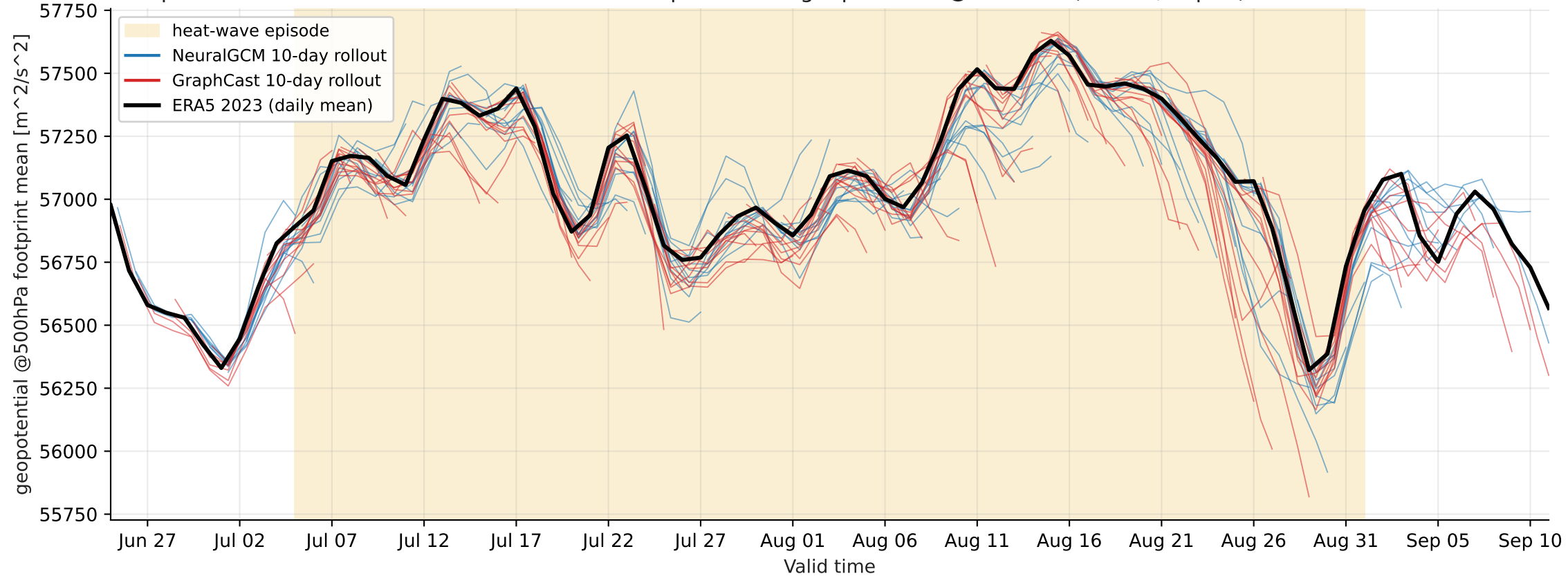
Europe heat-wave 2023-07-05..2023-09-01 — footprint-mean geopotential @ 500 hPa (cordex, > p99)
