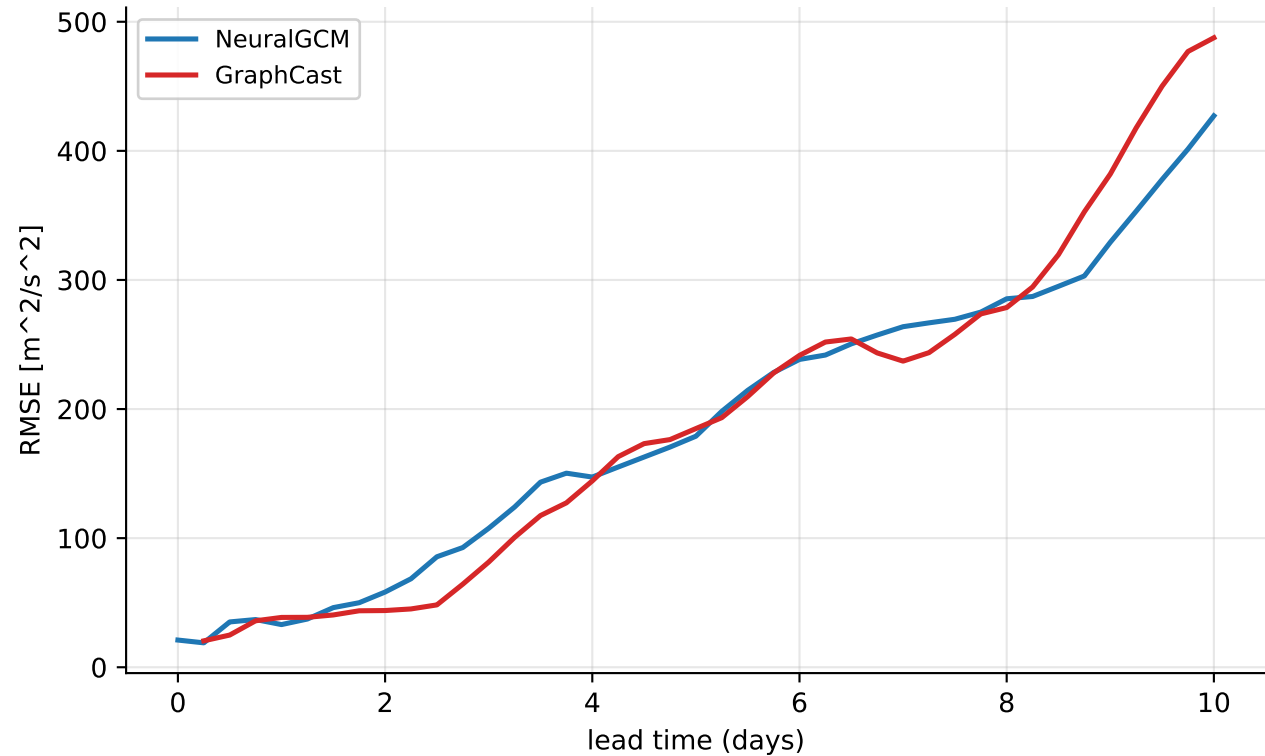
Europe heat-wave 2023-07-28..2023-08-04 — footprint geopotential@500 hPa (mean of 18 rollouts)
