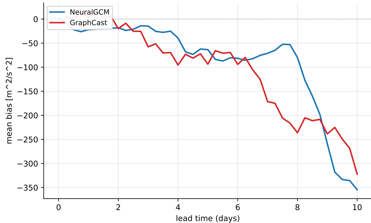
Europe heat-wave 2026-06-20..2026-06-27 — footprint geopotential@500 hPa (mean of 18 rollouts)
