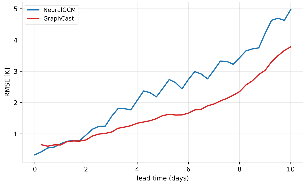
Europe heat-wave 2026-06-30..2026-07-24 — footprint temperature@850 hPa (mean of 23 rollouts)
