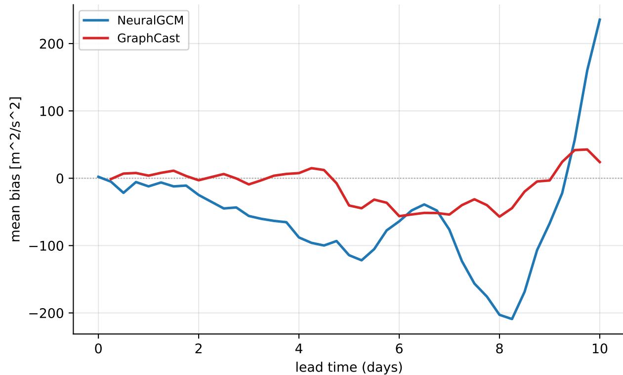
Europe heat-wave 2023-06-10..2023-06-21 — footprint geopotential@500 hPa (mean of 22 rollouts)
