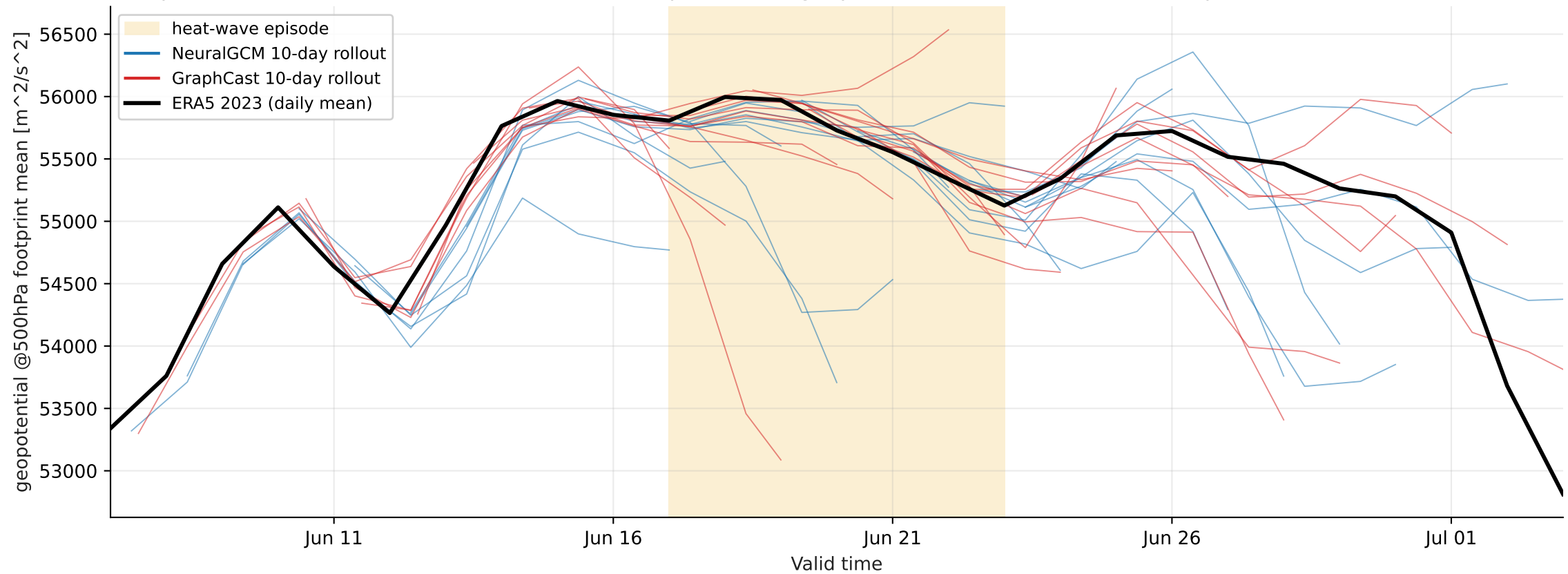
Europe heat-wave 2023-06-17..2023-06-23 — footprint-mean geopotential @ 500 hPa (mixture, > p99)
