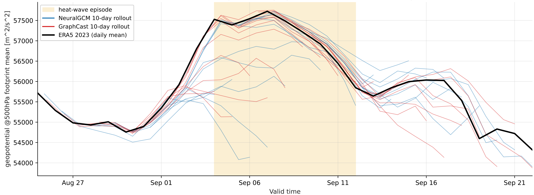
Europe heat-wave 2023-09-04..2023-09-12 — footprint-mean geopotential @ 500 hPa (mixture, > p99)
