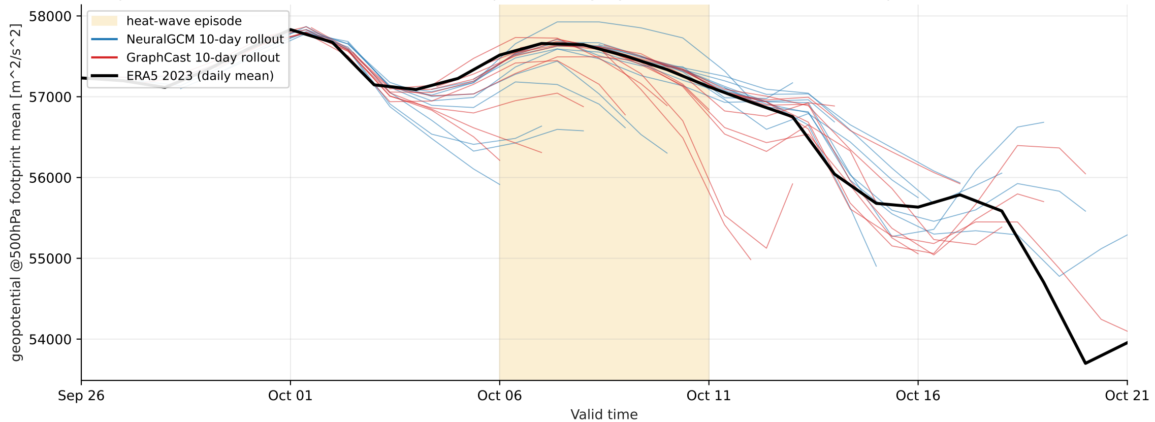
Europe heat-wave 2023-10-06..2023-10-11 — footprint-mean geopotential @ 500 hPa (mixture, > p99)
