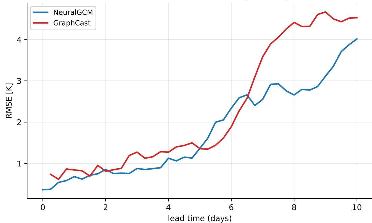
Europe heat-wave 2026-02-21..2026-02-25 — footprint temperature@850 hPa (mean of 15 rollouts)
