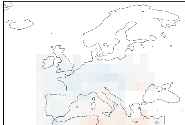
NeuralGCM
