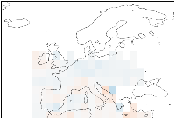
GraphCast
