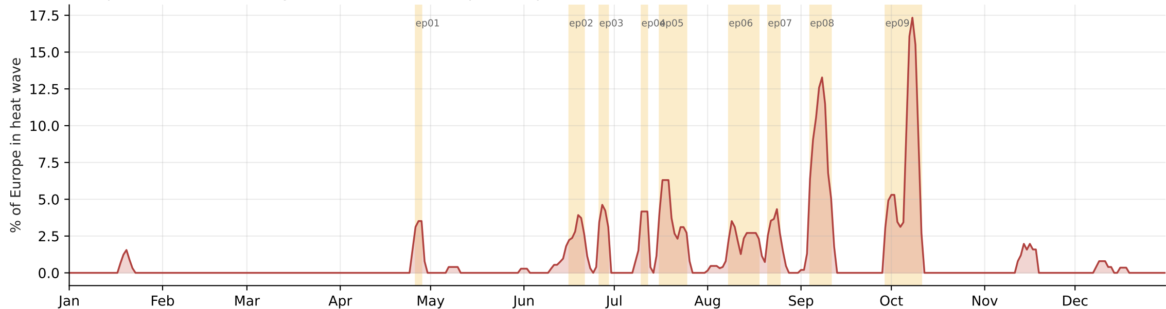
Europe heat-wave coverage in 2023 (mixture > p99, 9 episodes)
