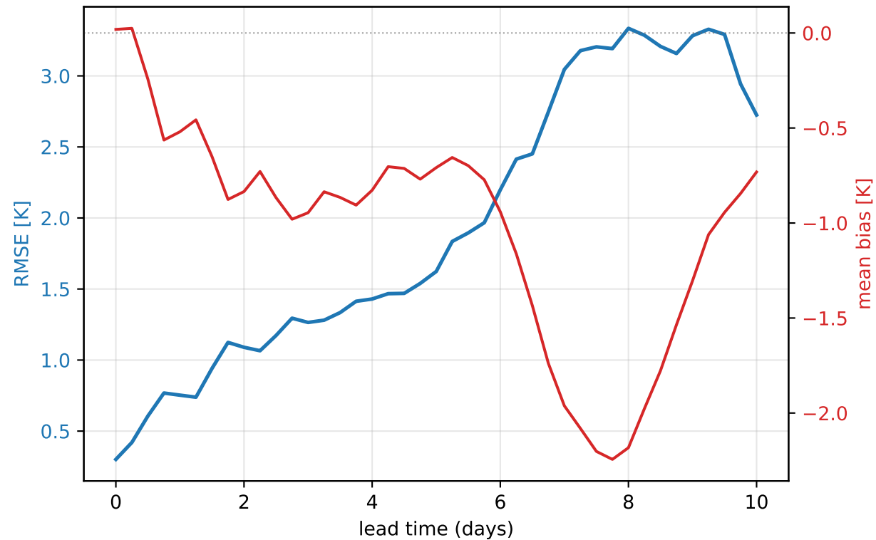
Europe heat-wave 2023-04-26..2023-04-28 — footprint temperature@850 hPa (mean of 13 rollouts)
