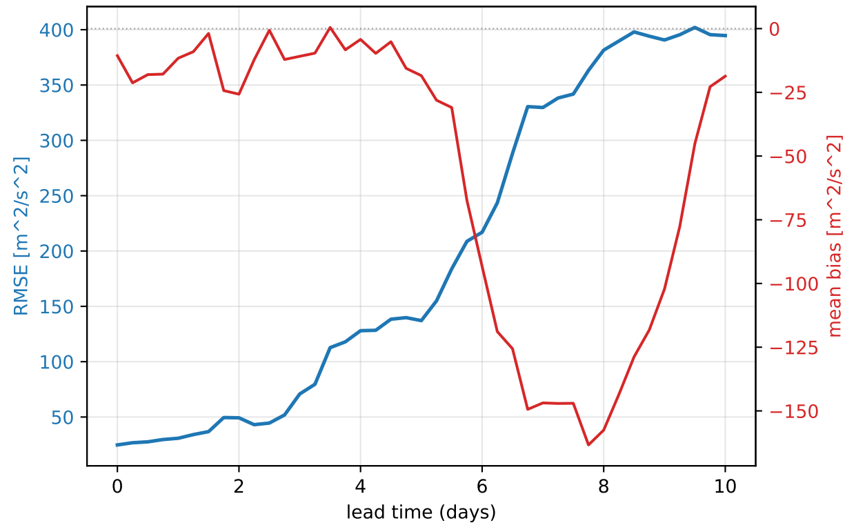
Europe heat-wave 2023-04-26..2023-04-28 — footprint geopotential@500 hPa (mean of 13 rollouts)
