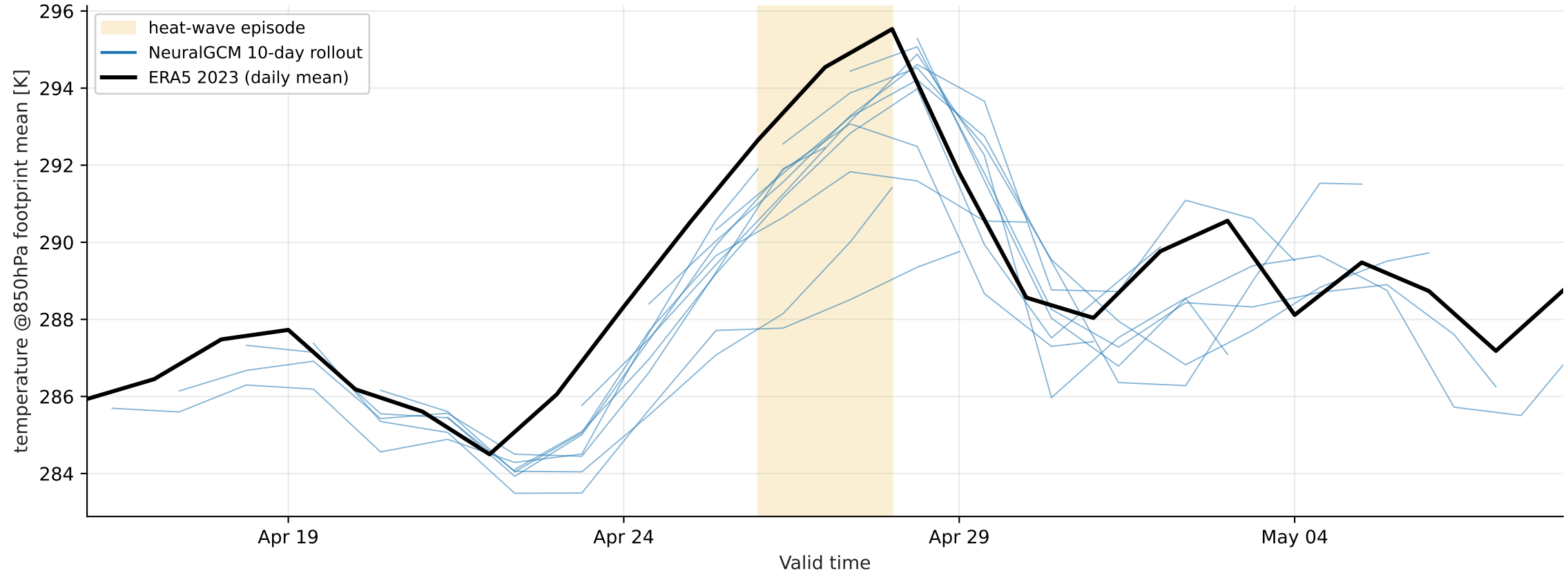
Europe heat-wave 2023-04-26..2023-04-28 — footprint-mean temperature @ 850 hPa (mixture, > p99)
