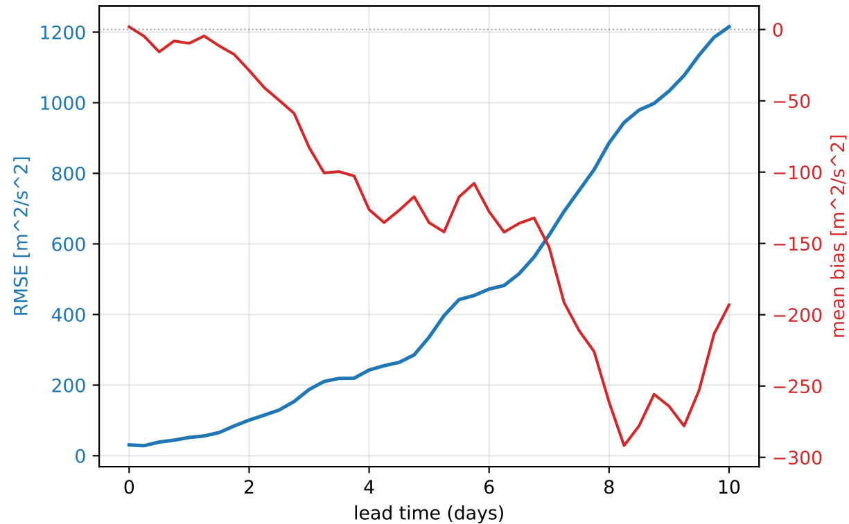
Europe heat-wave 2023-06-16..2023-06-21 — footprint geopotential@500 hPa (mean of 16 rollouts)
