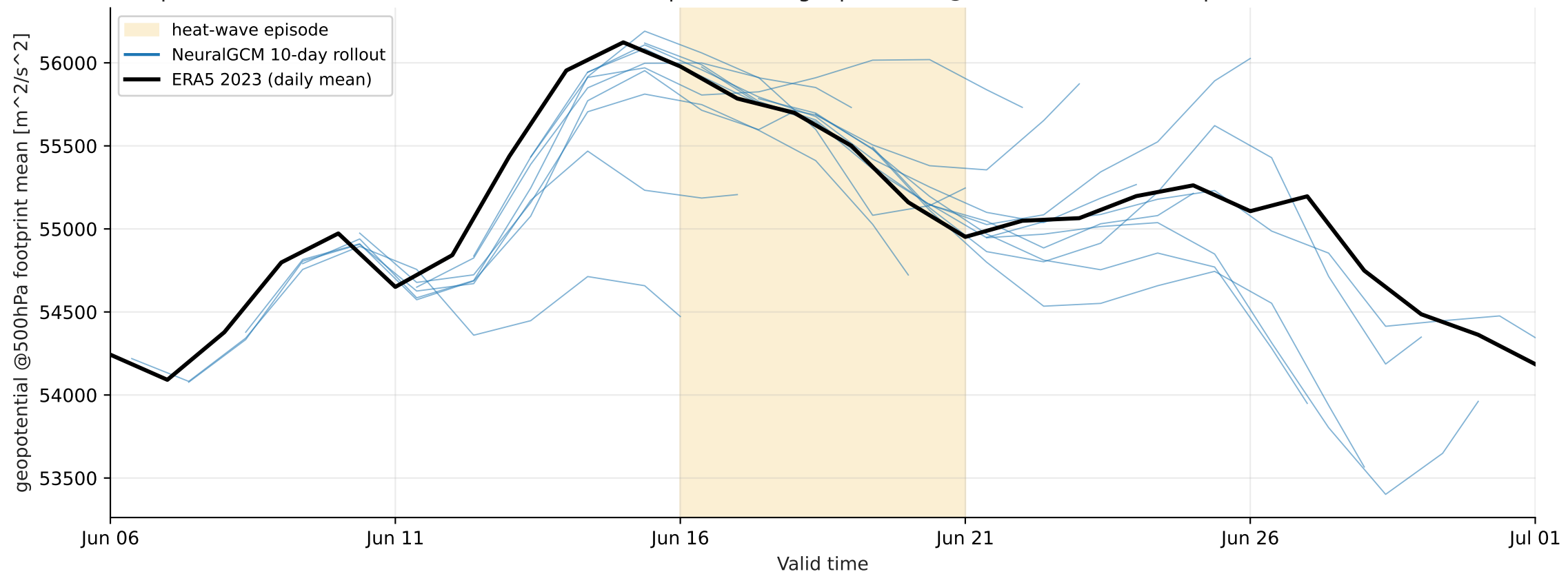
Europe heat-wave 2023-06-16..2023-06-21 — footprint-mean geopotential @ 500 hPa (mixture, > p99)
