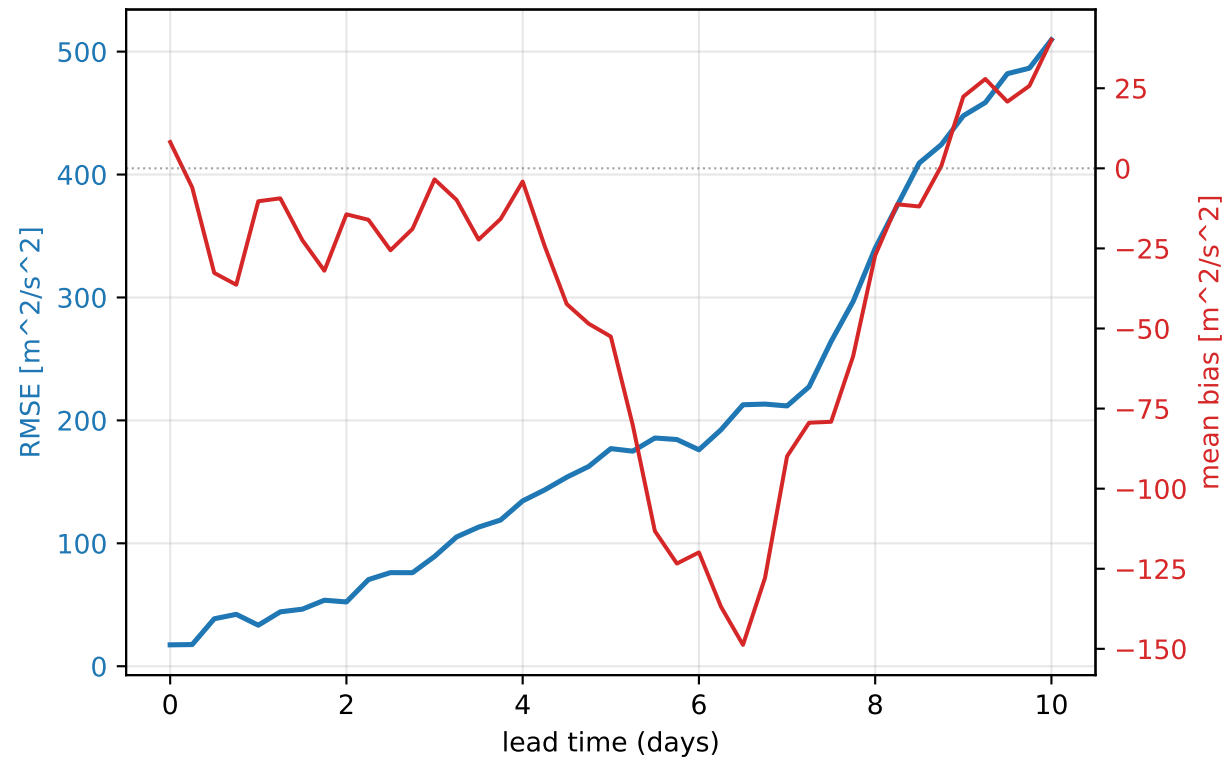
Europe heat-wave 2023-06-26..2023-06-29 — footprint geopotential@500 hPa (mean of 14 rollouts)
