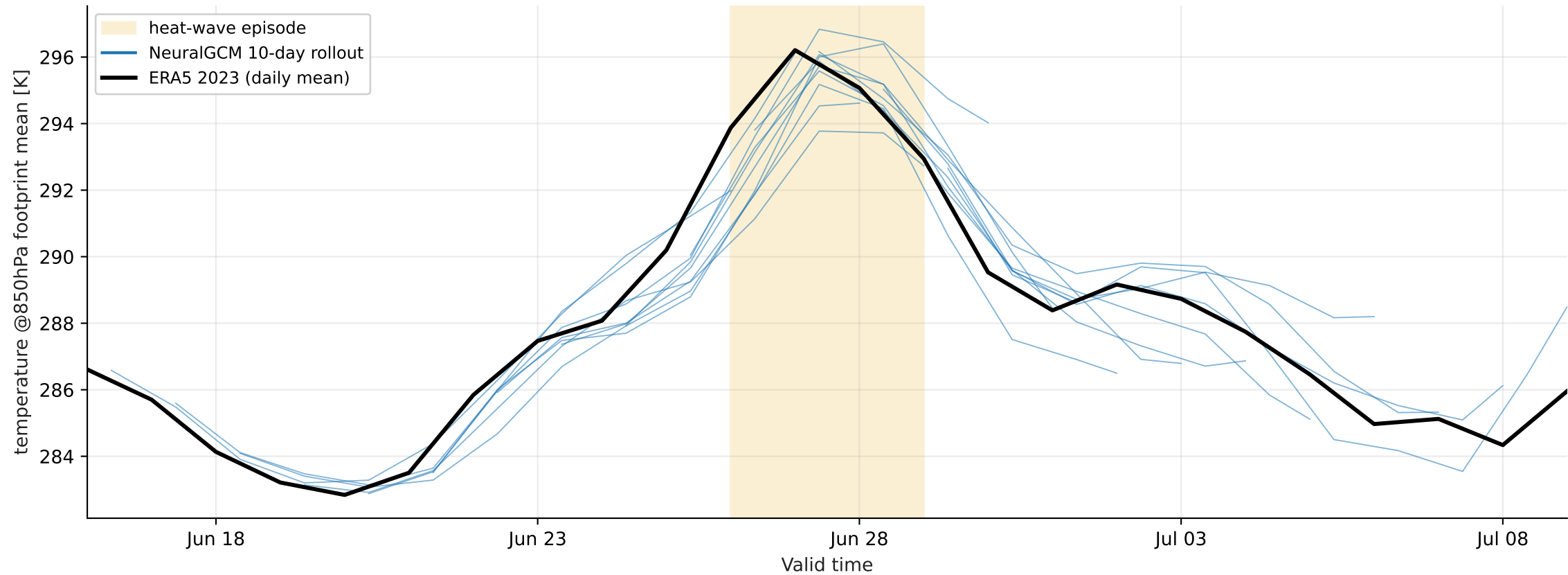
Europe heat-wave 2023-06-26..2023-06-29 — footprint-mean temperature @ 850 hPa (mixture, > p99)
