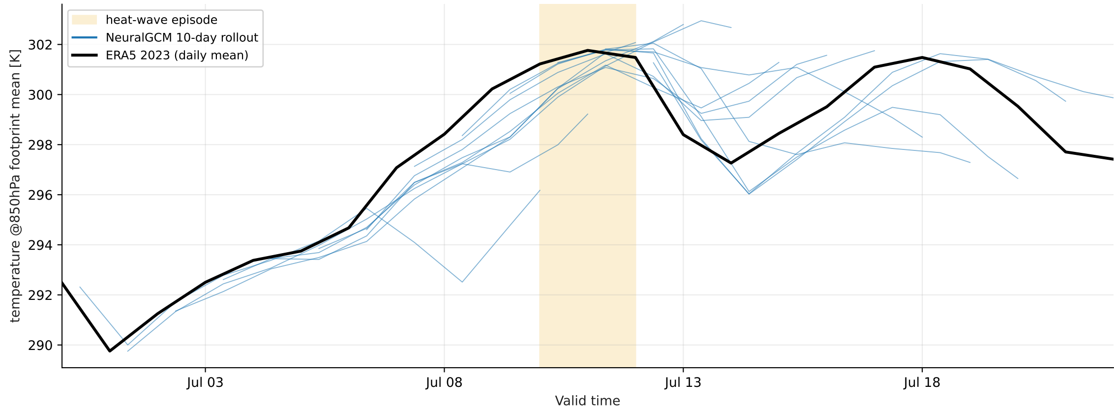
Europe heat-wave 2023-07-10..2023-07-12 — footprint-mean temperature @ 850 hPa (mixture, > p99)
