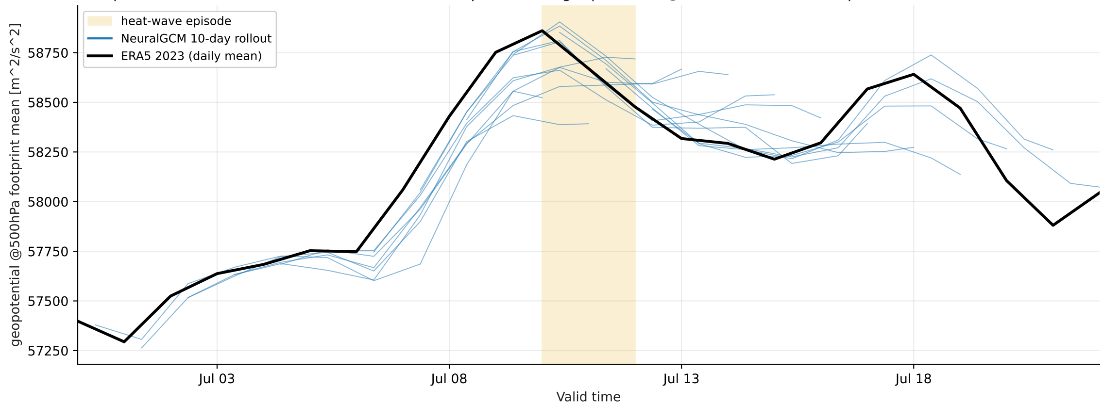
Europe heat-wave 2023-07-10..2023-07-12 — footprint-mean geopotential @ 500 hPa (mixture, > p99)
