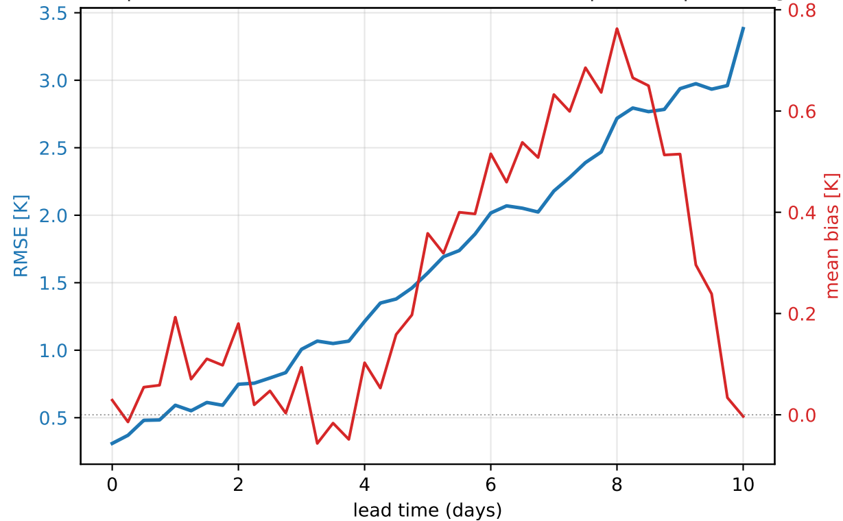
Europe heat-wave 2023-07-16..2023-07-25 — footprint temperature@850 hPa (mean of 20 rollouts)
