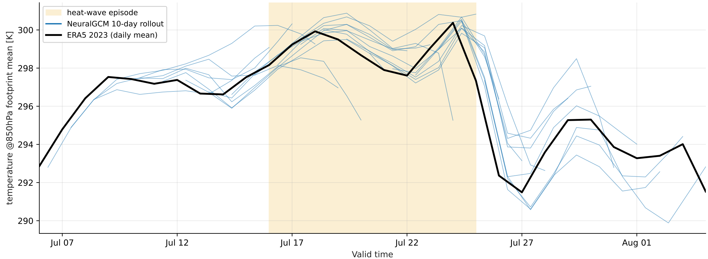
Europe heat-wave 2023-07-16..2023-07-25 — footprint-mean temperature @ 850 hPa (mixture, > p99)
