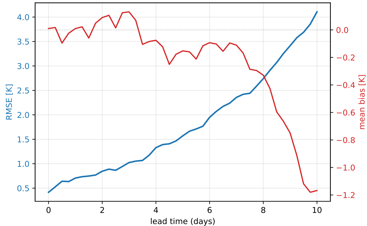
Europe heat-wave 2023-08-08..2023-08-18 — footprint temperature@850 hPa (mean of 21 rollouts)
