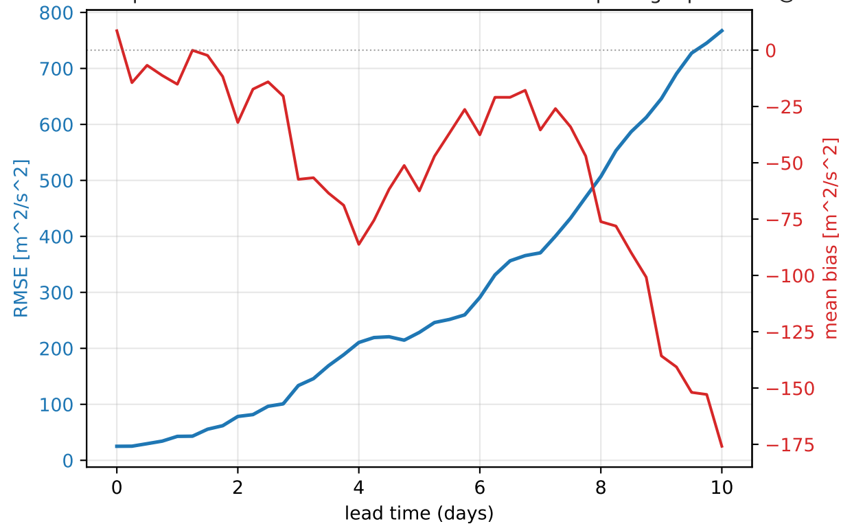
Europe heat-wave 2023-08-08..2023-08-18 — footprint geopotential@500 hPa (mean of 21 rollouts)
