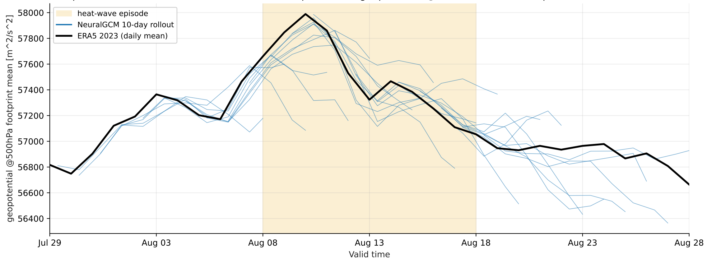
Europe heat-wave 2023-08-08..2023-08-18 — footprint-mean geopotential @ 500 hPa (mixture, > p99)
