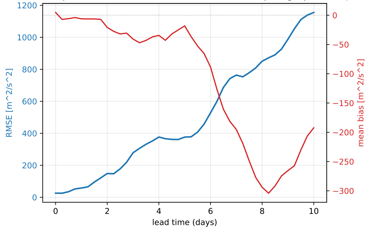
Europe heat-wave 2023-08-21..2023-08-25 — footprint geopotential@500 hPa (mean of 15 rollouts)
