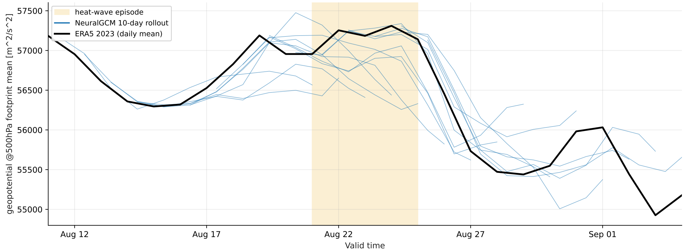
Europe heat-wave 2023-08-21..2023-08-25 — footprint-mean geopotential @ 500 hPa (mixture, > p99)
