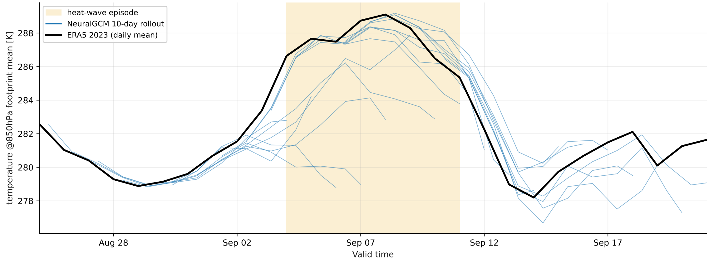
Europe heat-wave 2023-09-04..2023-09-11 — footprint-mean temperature @ 850 hPa (mixture, > p99)
