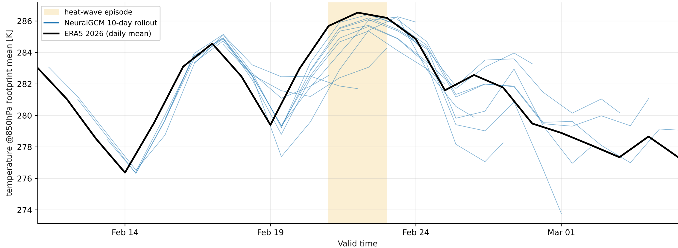
Europe heat-wave 2026-02-21..2026-02-23 — footprint-mean temperature @ 850 hPa (mixture, > p99)
