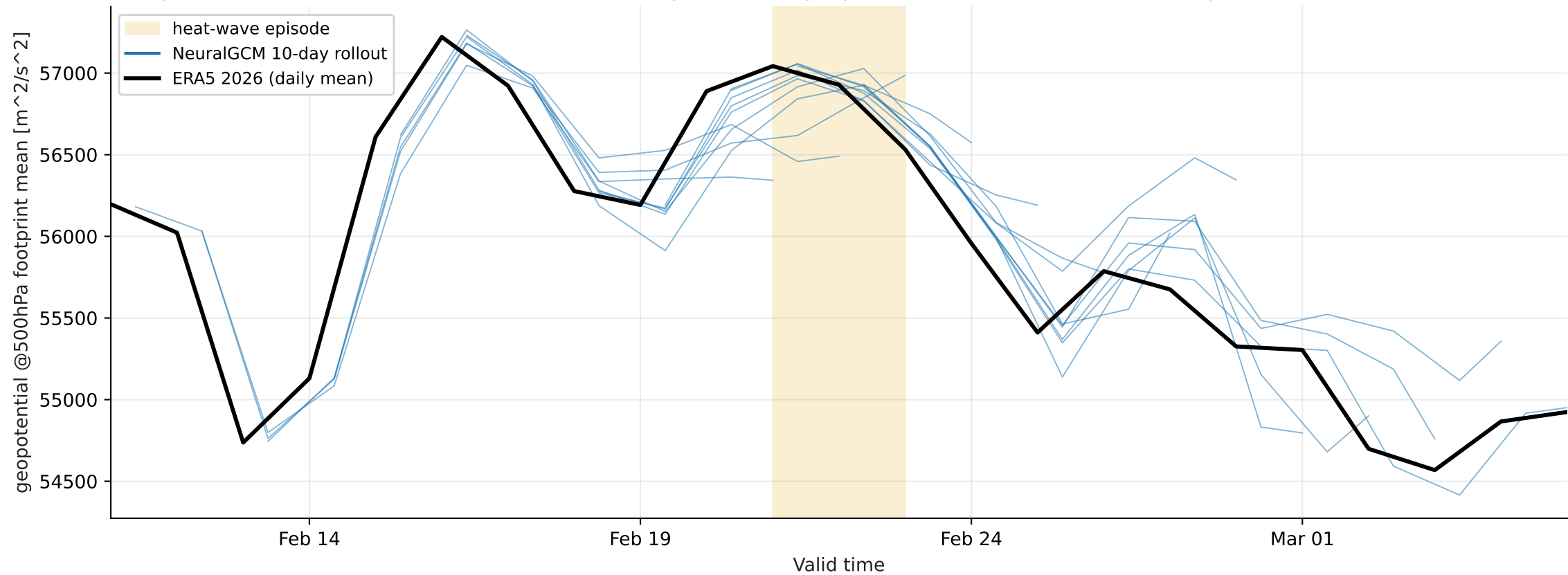
Europe heat-wave 2026-02-21..2026-02-23 — footprint-mean geopotential @ 500 hPa (mixture, > p99)
